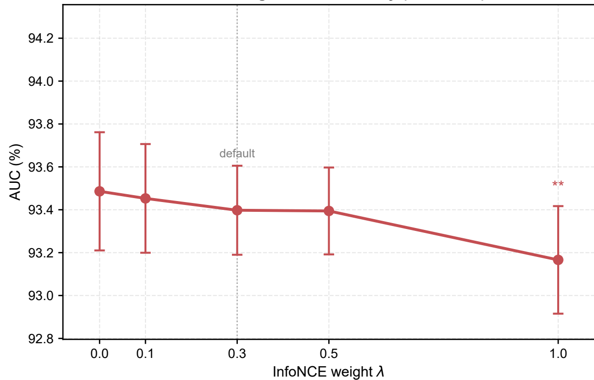
InfoNCE Alignment Sensitivity (TwiBot-20)
