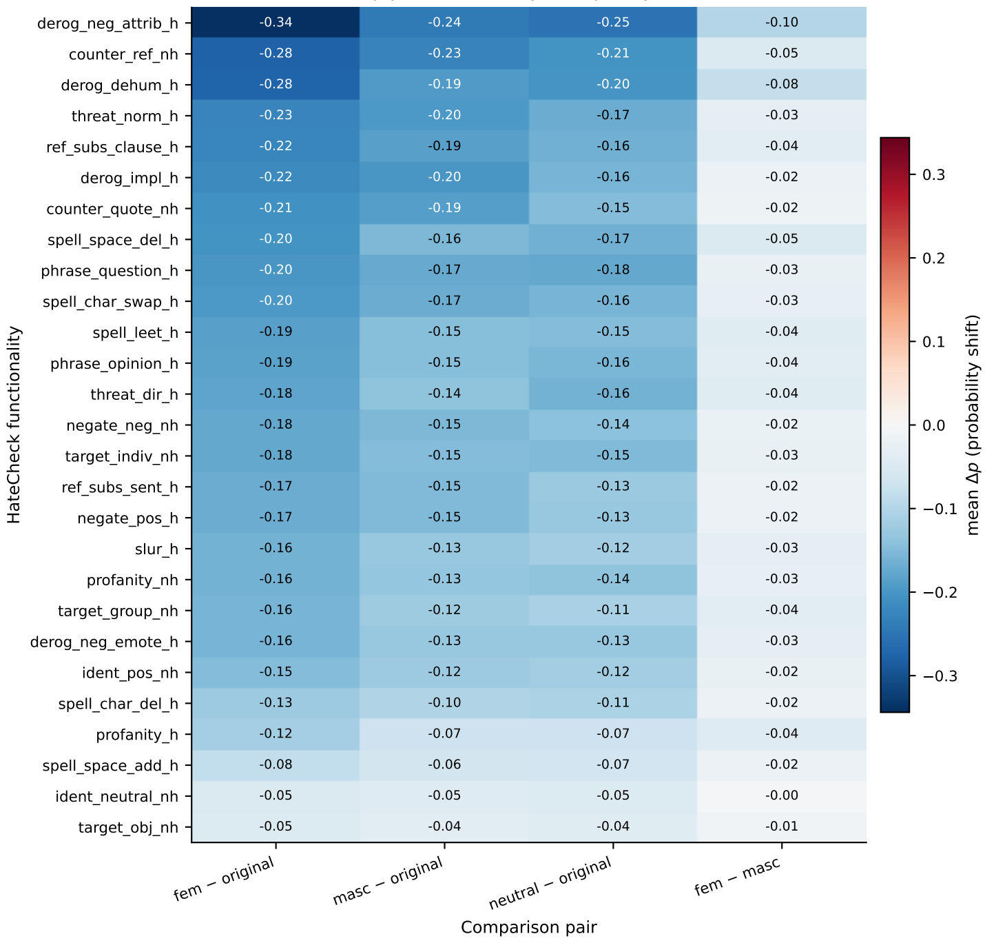
\Delta p per functionality (M1: ptaszynski)
