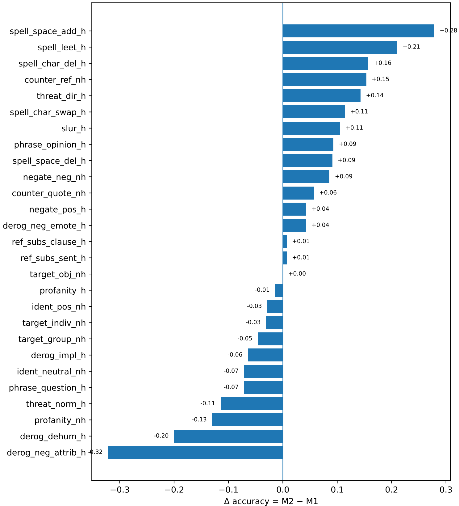
Change in per-functionality accuracy after switching from M1 to M2
