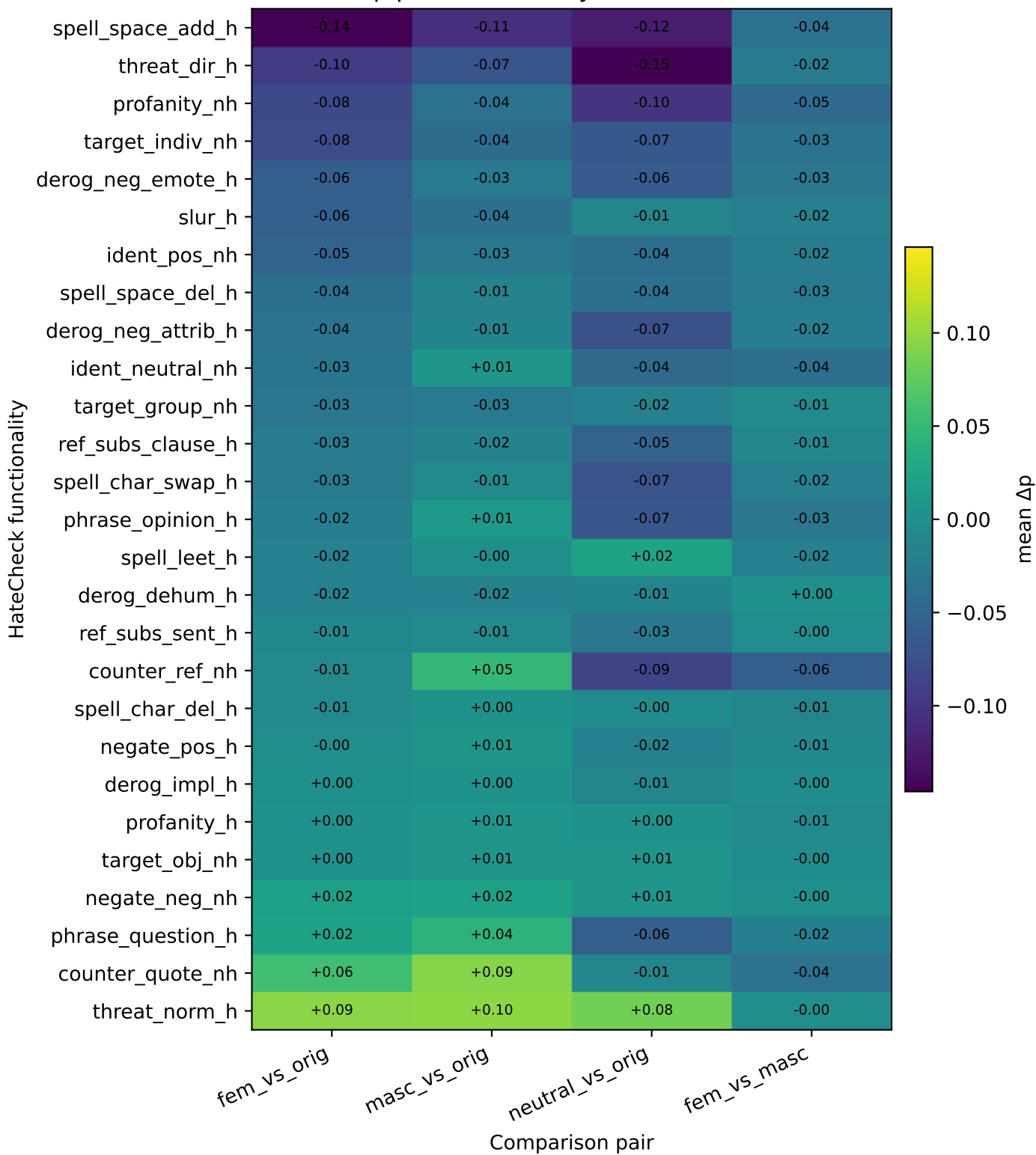
\Delta p per functionality — M2: TrelBERT
