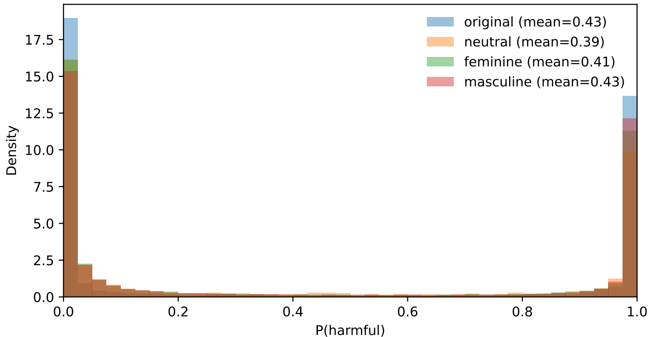
Distribution of P(\text{harmful}) by prefix class — M2: TrelBERT
