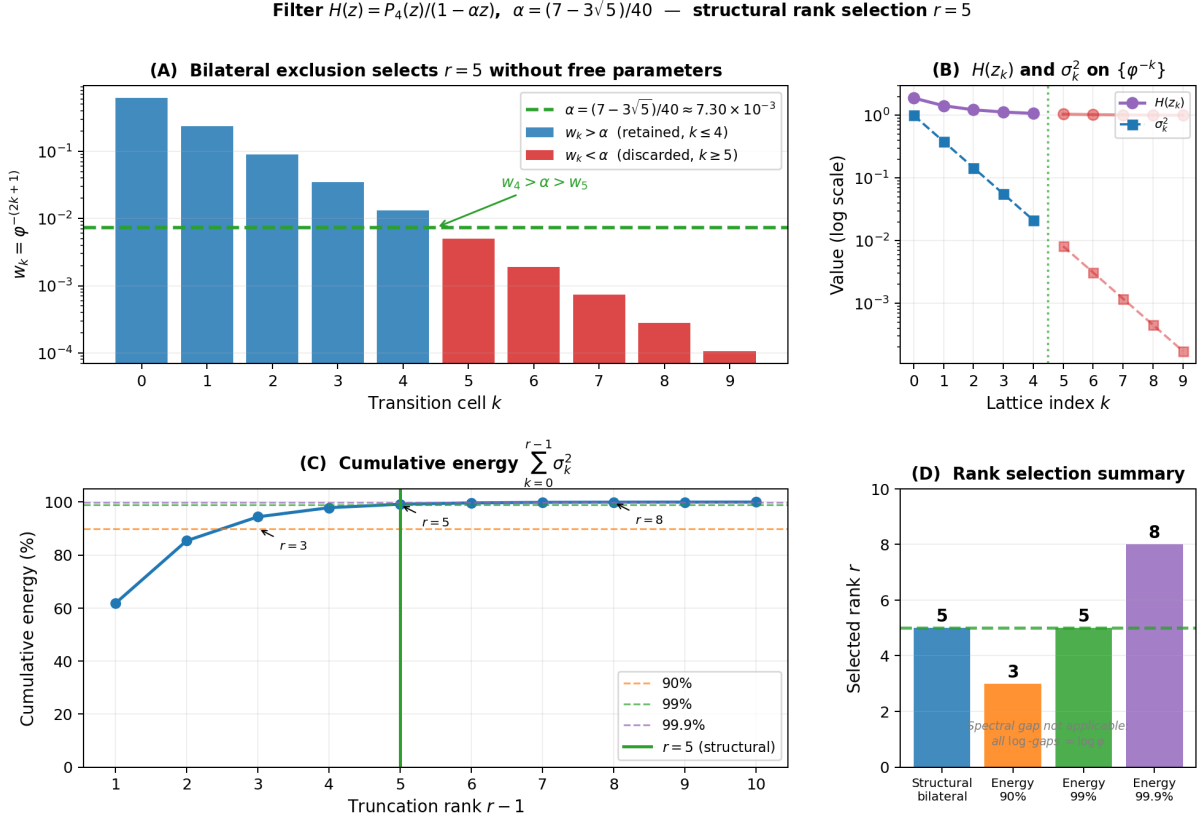
Figure 5: Numerical verification of the rank-selection criterion. (A) Transition weights w_k = \varphi^{-(2k+1)} on logarithmic scale; dashed line: threshold \alpha = (7 - 3\sqrt{5})/40 . The bilateral exclusion w_4 > \alpha > w_5 is exact. (B) Filter values H(z_k) and metric weights \sigma_k^2 on the autosimilar lattice \{z_k = \varphi^{-k}\} ; both decay monotonically with a natural cutoff at k = 5 . (C) Cumulative spectral energy: the 99% level coincides with r = 5 , while 90% selects r = 3 and 99.9% selects r = 8 . (The spectral gap criterion is not applicable here: all log-gaps equal \log \varphi , so no gap is larger than any other.) (D) Summary: the structural bilateral exclusion and the 99% energy threshold both select r = 5 ; the empirical choice is unstable with respect to the threshold level, while the structural method requires no free parameter.
