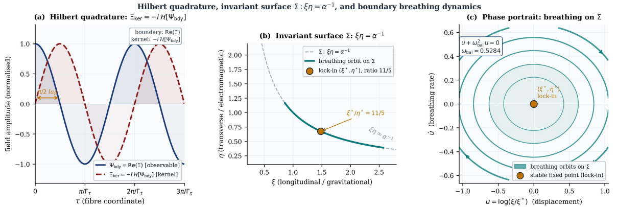
Figure 1: Hilbert quadrature, invariant surface, and boundary breathing dynamics. (a) The observable boundary field \Psi_{\text{bdy}} = \text{Re}(\Xi) and the kernel quadrature \Xi_{\text{ker}} = -i \mathcal{H}[\Psi_{\text{bdy}}] form a Hilbert pair on the compact fibre S^1(\tau) : the boundary sees the real part of the bulk Majorana field; the kernel carries its Hilbert transform. (b) The two chiral channels (\xi, \eta) live on the invariant hyperbolic surface \Sigma: \xi \eta = \alpha^{-1} . The breathing orbit (teal) oscillates on \Sigma around the lock-in point (\xi^*, \eta^*) with ratio \xi^*/\eta^* = 11/5 . (c) Phase portrait of the breathing equation \ddot{u} + \omega_{\text{bal}}^2 u = 0 , u := \log(\xi/\xi^*) , \omega_{\text{bal}} = 0.5284 . The stable fixed point at the origin is the lock-in; the closed orbits are the boundary breathing modes. The fine-structure constant \alpha^{-1} is the conserved invariant of this projected exchange, not an externally inserted parameter.
