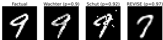
Figure 1: Turning a 9 into a 7: Counterfactual explanations for an image classifier produced using Wachter (Wachter et al. 2017), Schut (Schut et al. 2021) and REVISE (Joshi et al. 2019).
