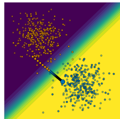
Figure 2: Gradient-based counterfactual search.
