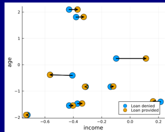
Figure 2: Counterfactuals for random samples from the Give Me Some Credit dataset (Kaggle 2011). Features ‘age’ and ‘income’ are shown.
