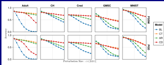
Figure 7: Test accuracies on adversarially perturbed data with varying perturbation sizes.
