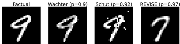
Figure 8: Turning a 9 into a 7: Counterfactual explanations for an image classifier produced using Wachter (Wachter et al. 2017), Schut (Schut et al. 2021) and REVISE (Joshi et al. 2019).
