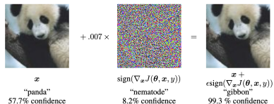
Figure 13: Example of an adversarial attack. Source: Goodfellow et al. (2015)
