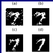
Figure 2: Turning a 9 into a 7. ECCC applied to MLP (a), Ensemble (b), JEM (c), JEM Ensemble (d).
