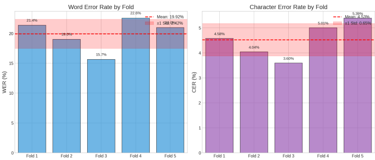
Gambar 4.4 Cross-Validation Summary — Freeze Encoder
