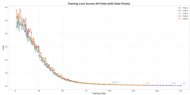
Gambar 4.2 Kurva Training Loss — Strategi LoRA
