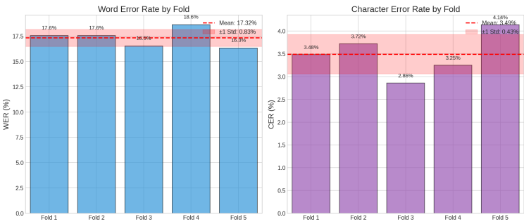
Gambar 4.5 Cross-Validation Summary — LoRA
