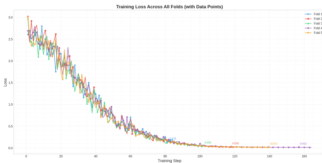
Gambar 4.1 Kurva Training Loss untuk 5-Fold Cross-Validation
