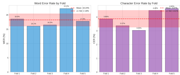
Gambar 4.6 Ringkasan Cross-Validation, Strategi Freeze Encoder (FE-9)
