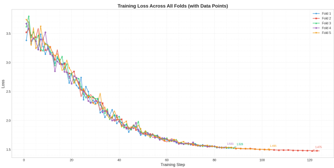
Gambar 4.1 Kurva Training Loss Strategi Freeze Encoder (FE-9)
