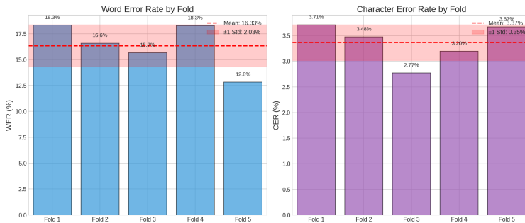
Gambar 4.6 Ringkasan Cross-Validation, Strategi LoRA (L-9)
