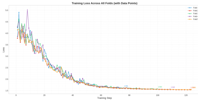
Gambar 4.3 Kurva Training Loss Strategi LoRA (L-9)
