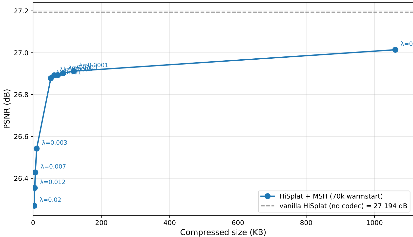
HiSplat + MSH RD curve (re10k test, 7286 scenes)
