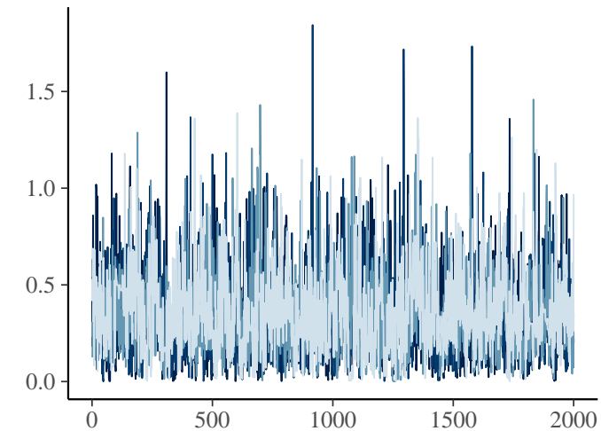
sigma_year
