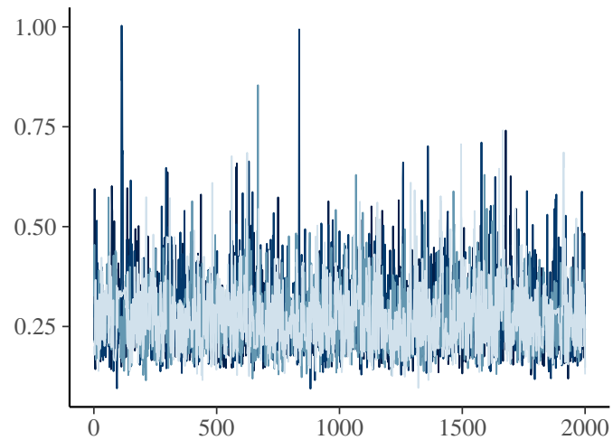
sigma_mu
