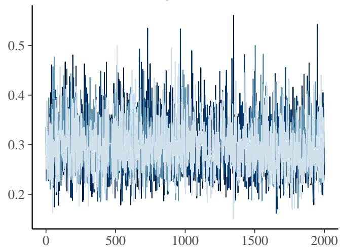
\sigma_{\mu}
