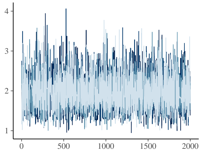
phi
