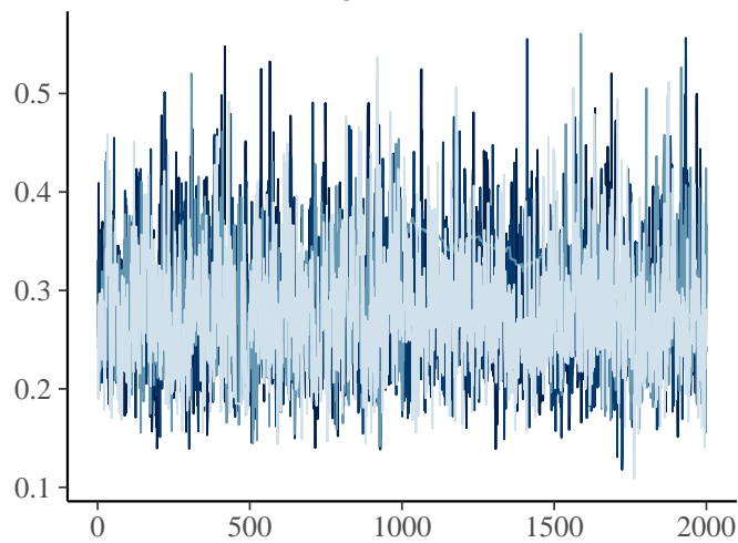
\sigma_{\text{width}}
