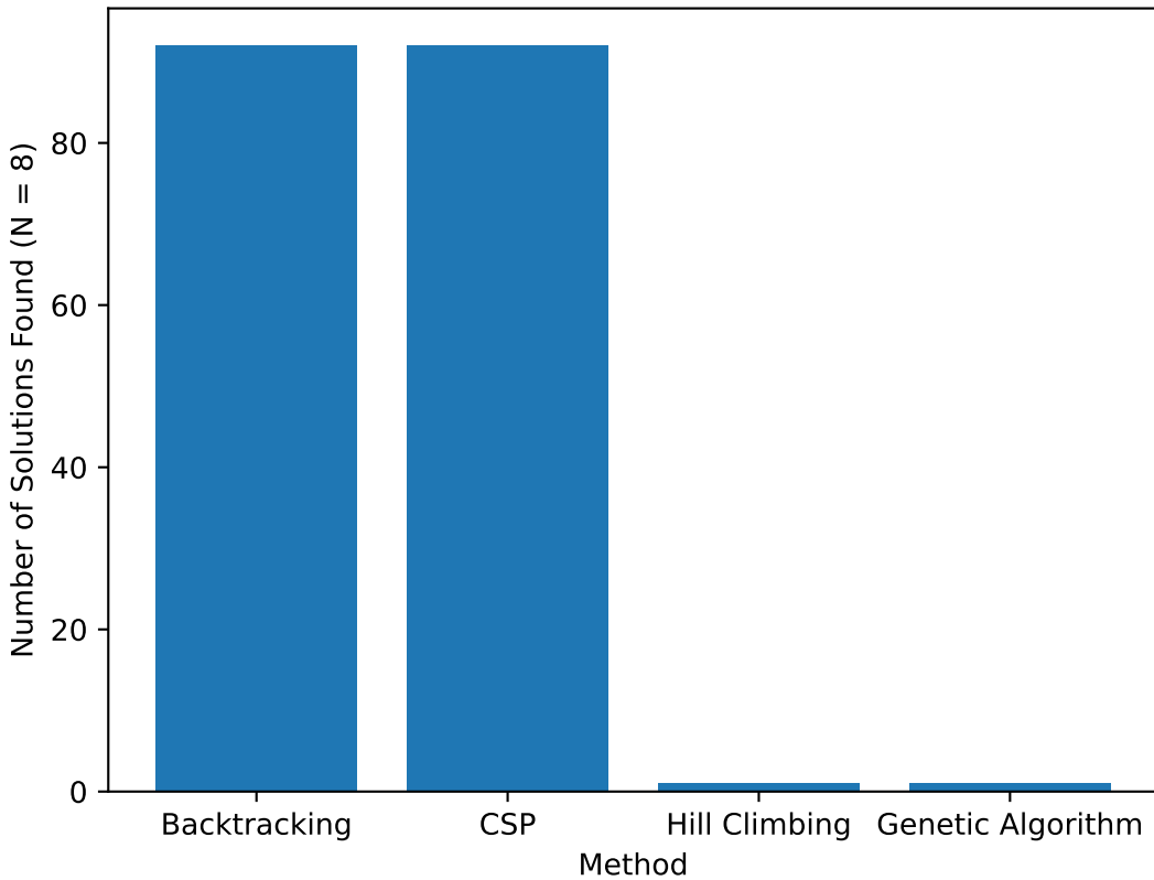
Solution Completeness Comparison Across Methods
