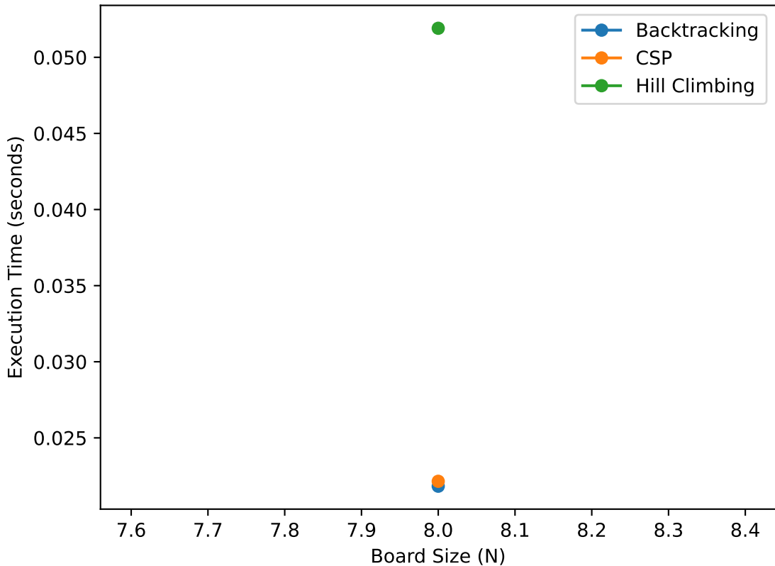
Scalability Analysis: Execution Time Growth with Board Size
