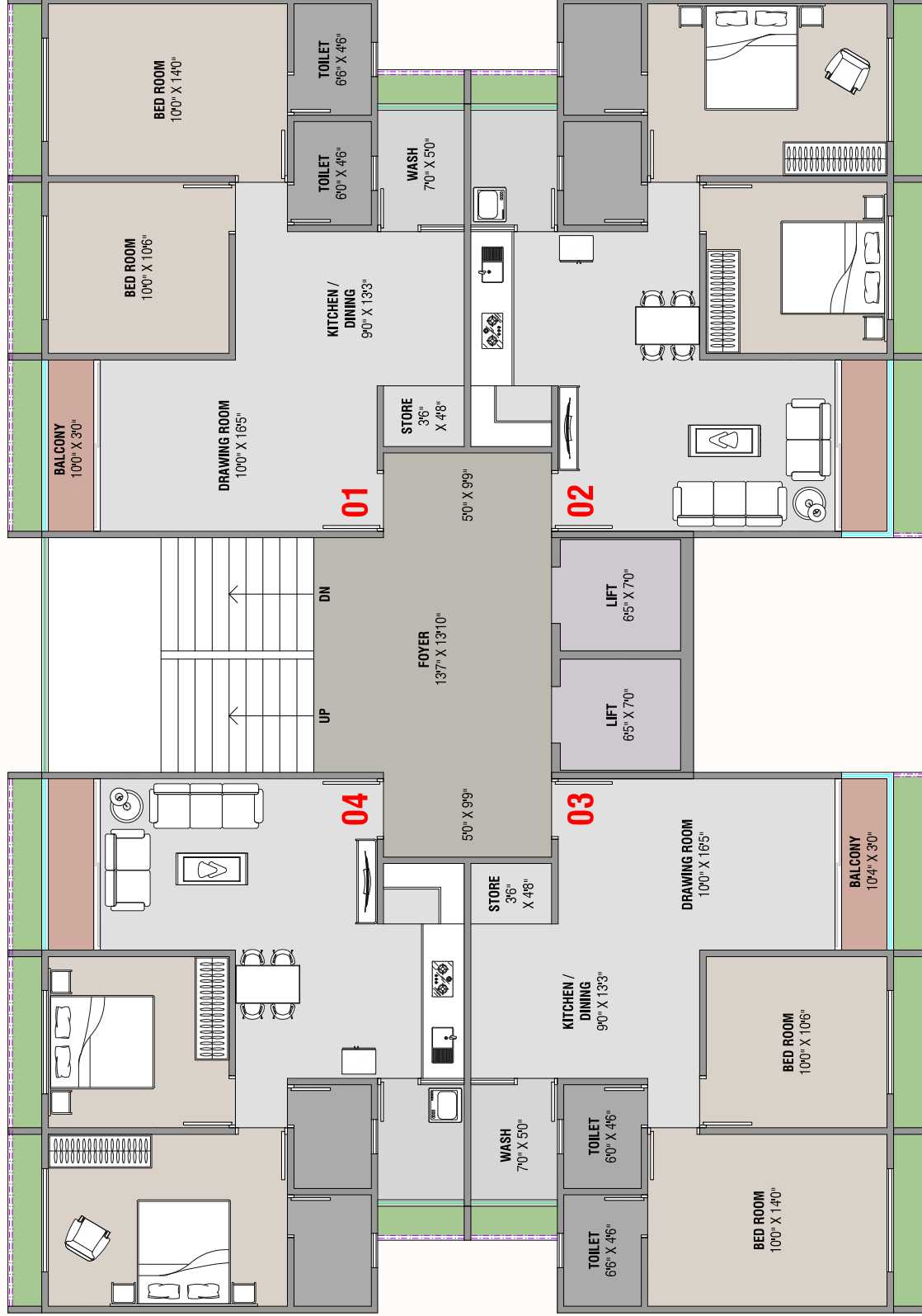
TYPICAL FLOOR PLAN (5TH TO 13TH) :- BLOCK - B
