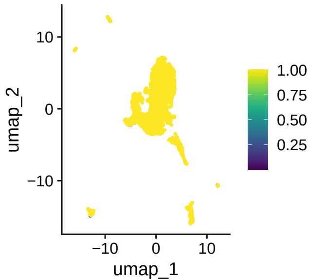
joint
