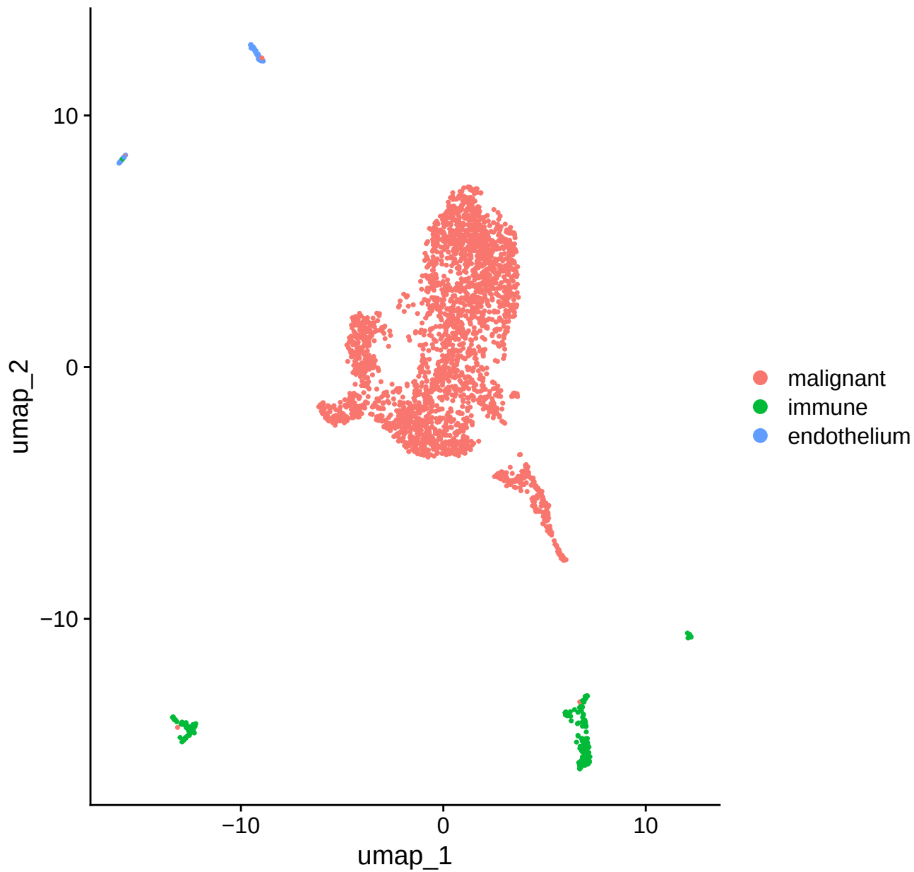
annotated_coarse
