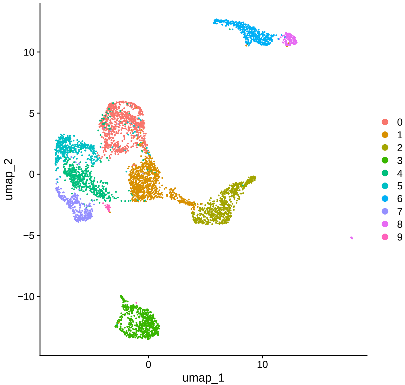
sample_cluster
