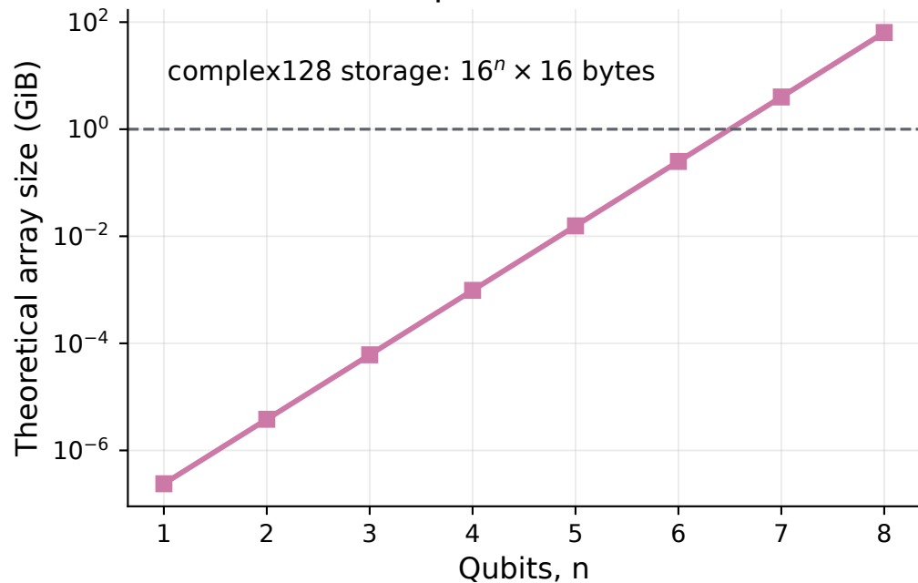
Exact-path Pauli tensor
