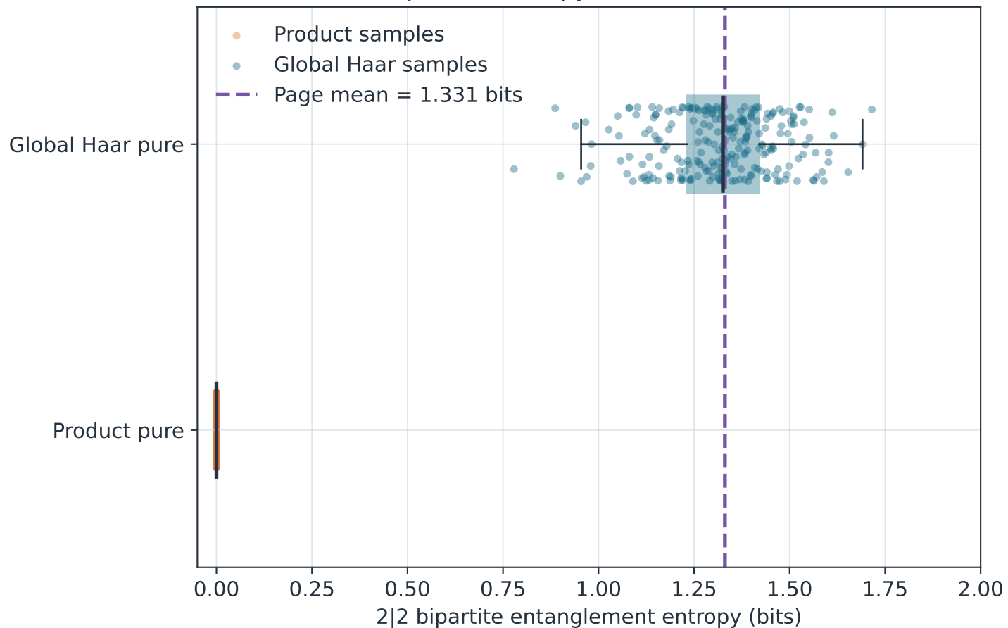
B Bipartite entropy distributions (n=4)
