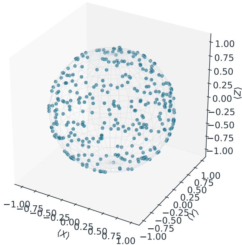
A Bloch-sphere samples
