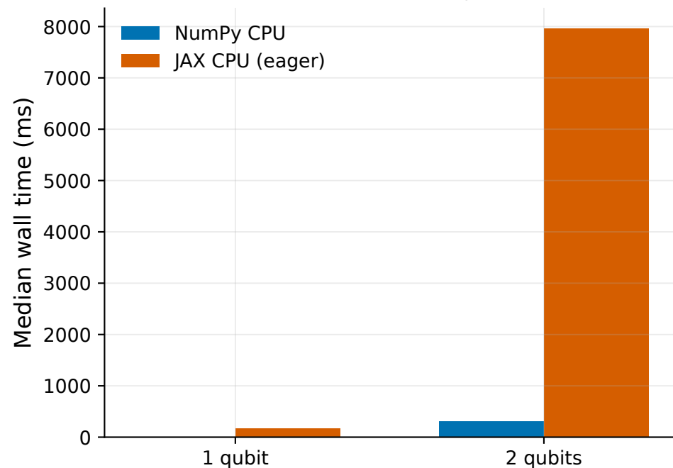
Same reconstruction code, two backends
