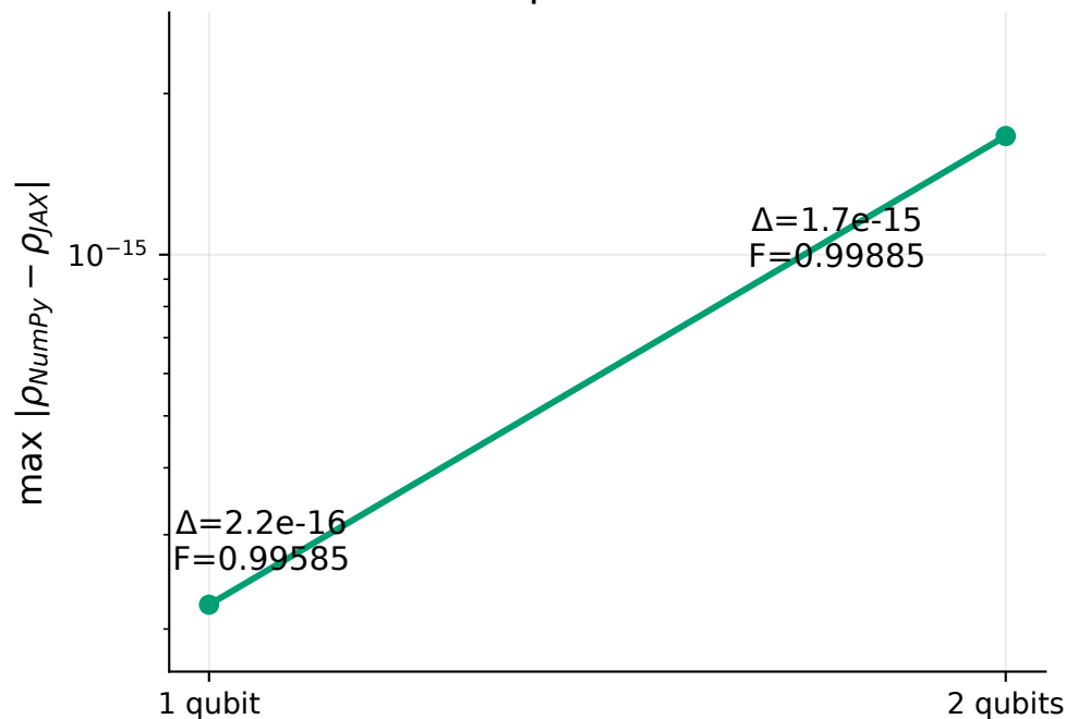
Fixed counts reproduce the same MLE
