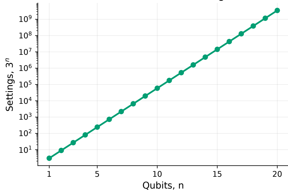
Exhaustive Pauli settings
