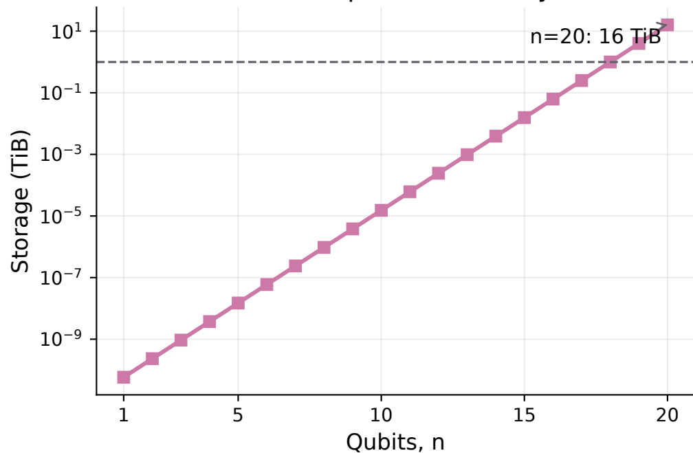
One dense complex128 density matrix
