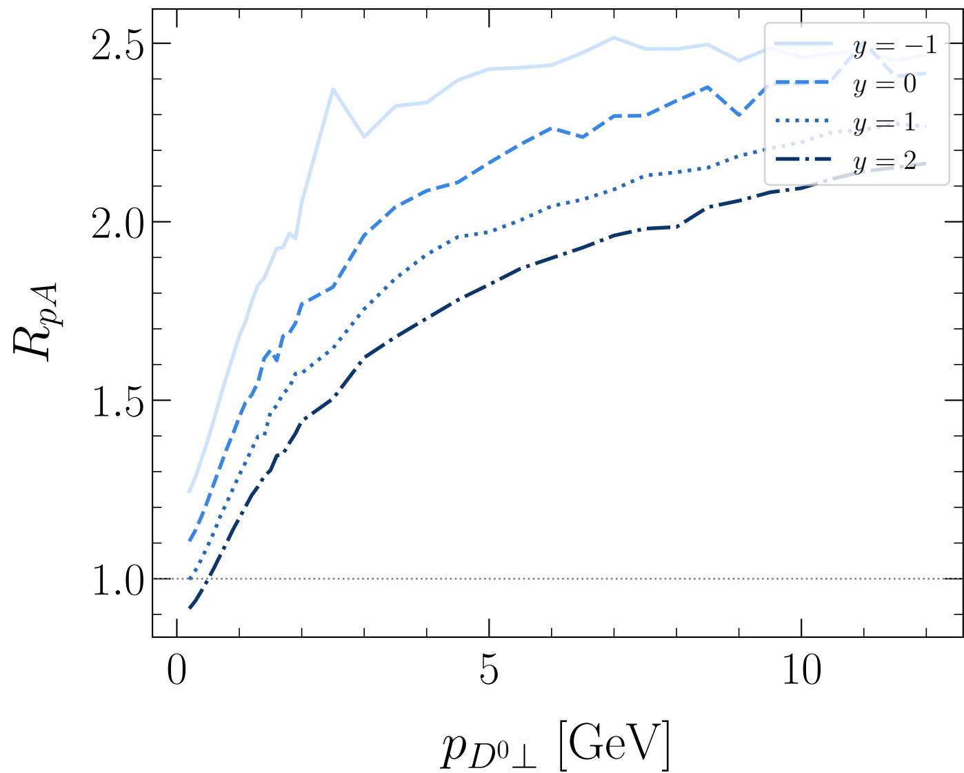
Nuclear modification factor R_{pA} (exclusive)
