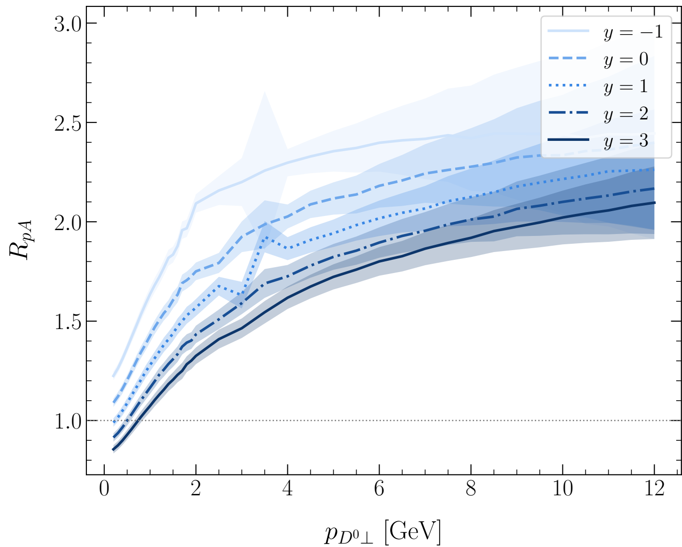
Nuclear modification factor R_{pA} (exclusive)
