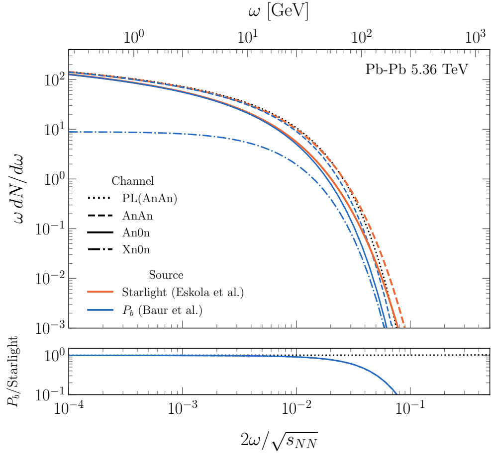
Figure 1: This code's simple single- b flux (Eq. 3) vs. the tabulated Starlight flux.
