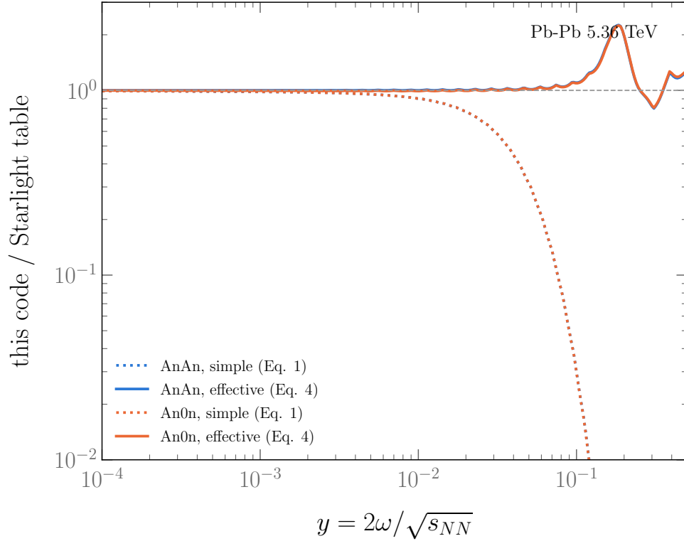
Figure 2: Ratio to the Starlight table: simple (dotted) vs. effective-flux (solid) treatment, for the AnAn and An0n channels.
