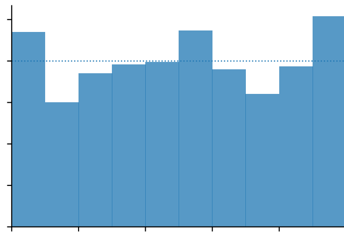
Matched constant variance
