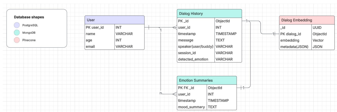
Figure 3.4 ER-Diagram for the Database
