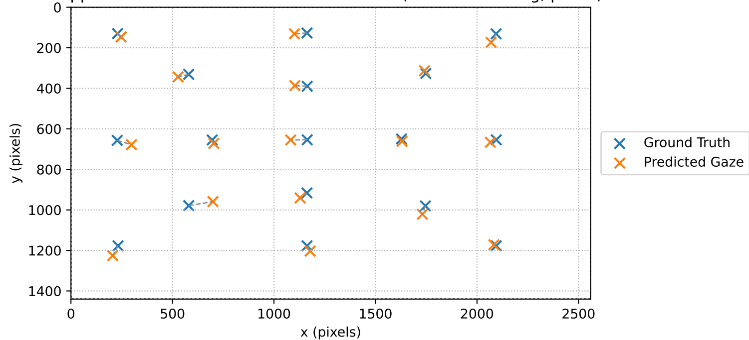
Approach 1 — Ground Truth vs Predictions (After Fine-Tuning, pixels)
