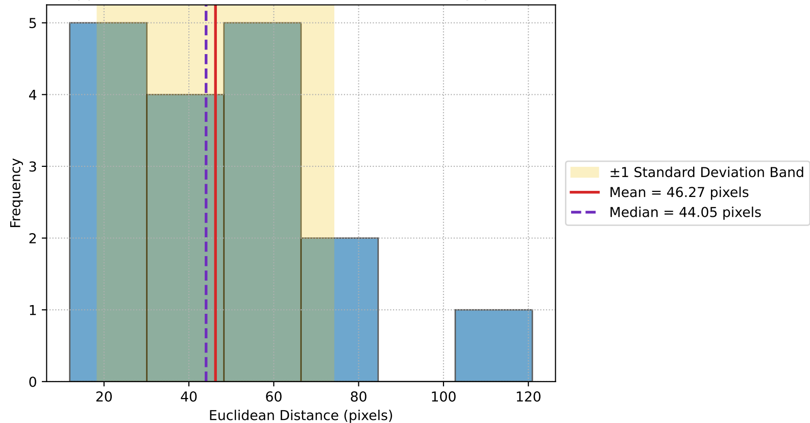
Approach 1 — Error Distribution (After Fine-Tuning, pixels)
