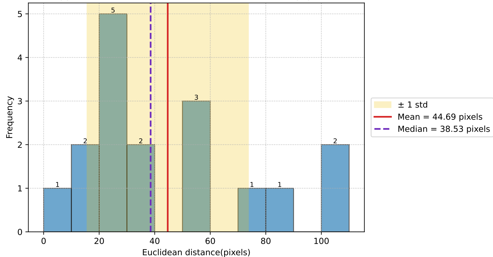
Approach 2 — Error Distribution (After Fine-Tuning, pixels)
