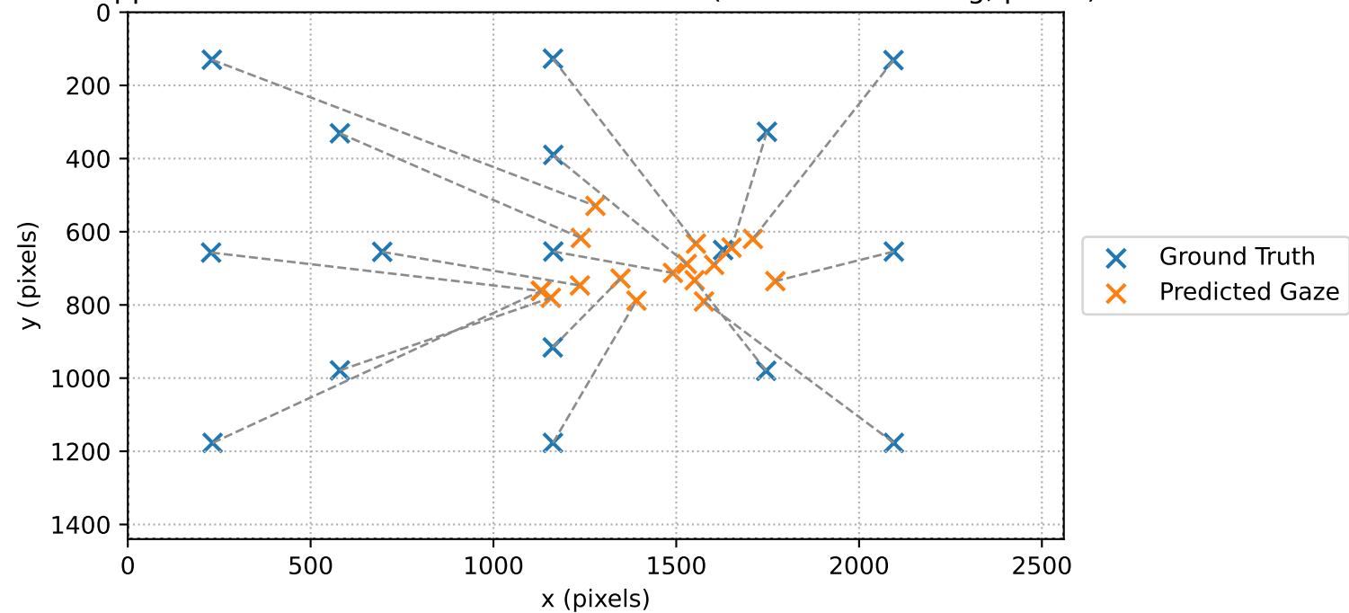
Approach 1 — Ground Truth vs Predictions (Before Fine-Tuning, pixels)
