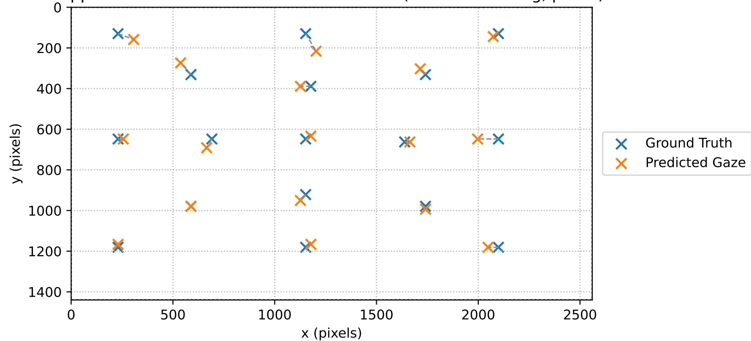
Approach 2 — Ground Truth vs Predictions (After Fine-Tuning, pixels)
