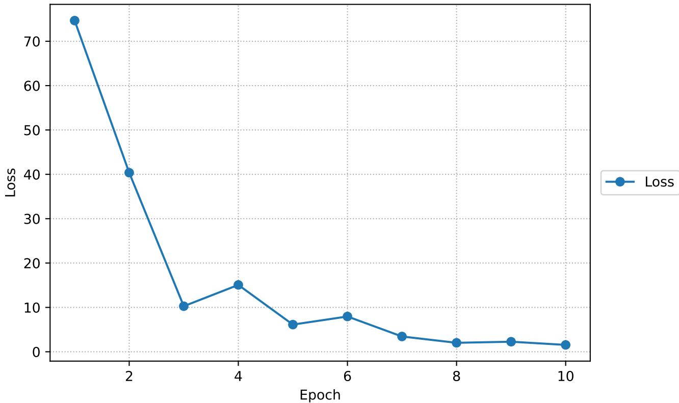
Approach 1 — Fine-Tuning Loss Curve
