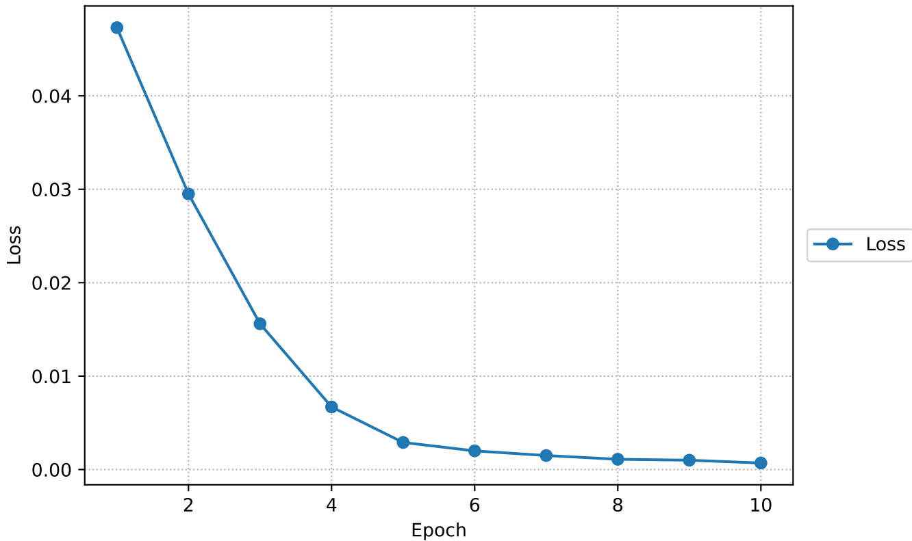
Approach 2 — Fine-Tuning Loss Curve
