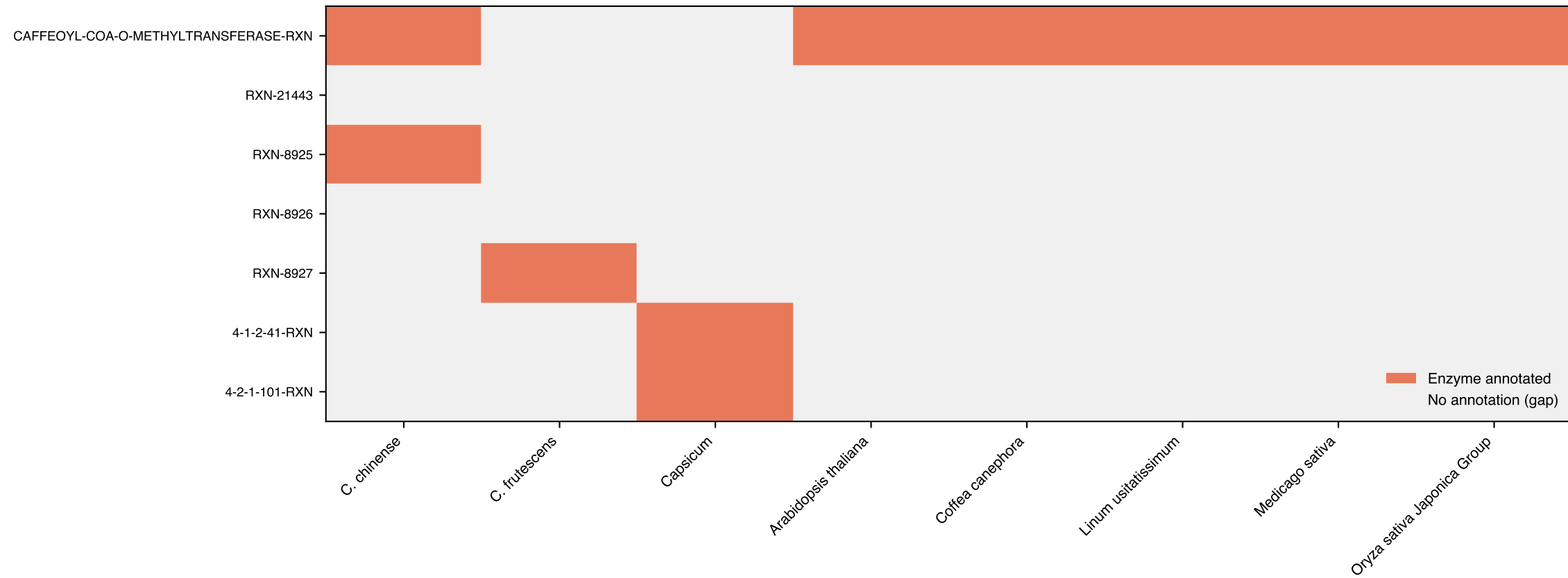
Reaction coverage in capsaicin biosynthesis (PC629) per species (orange = enzyme annotated, grey = no annotation / gap)
