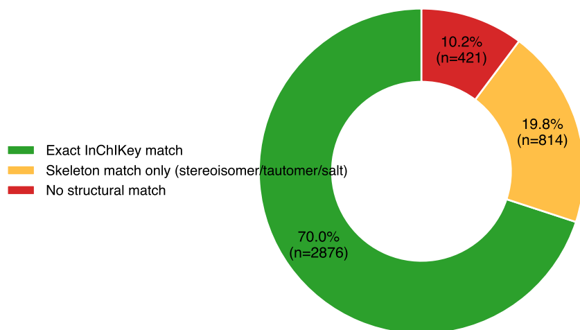
A. Wikidata coverage of all 4,111 InChIKey-annotated metabolites
