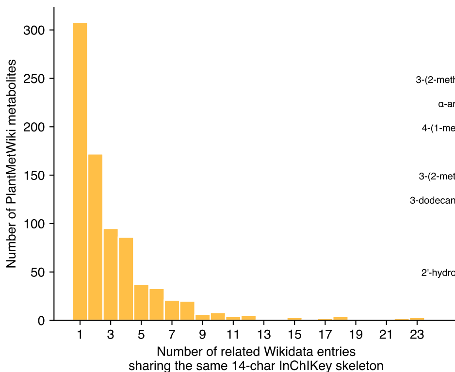
C. Chemical diversity already in Wikidata for the 814 skeleton-matched metabolites
