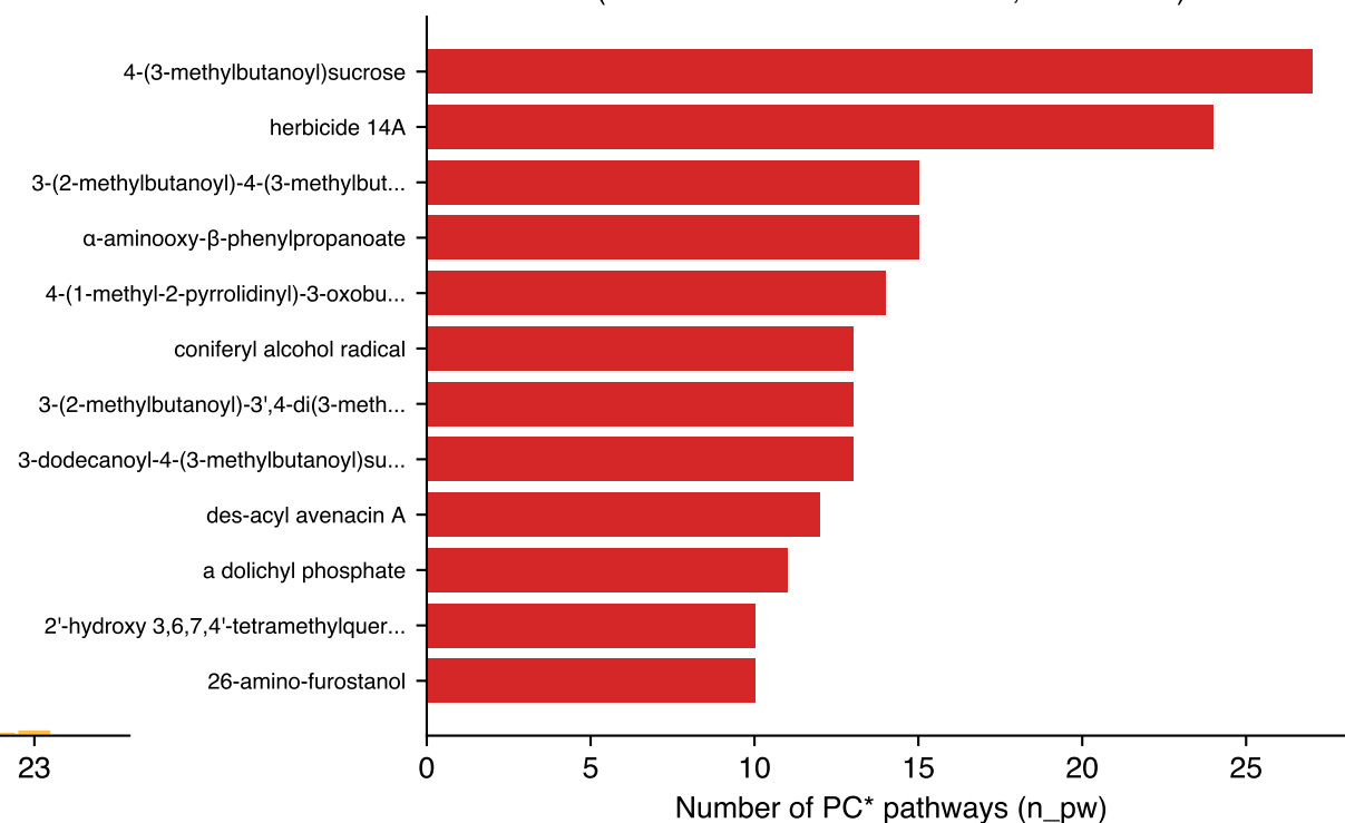
D. Spotlight: genuinely novel metabolites (no structural match in Wikidata, n=421 total)
