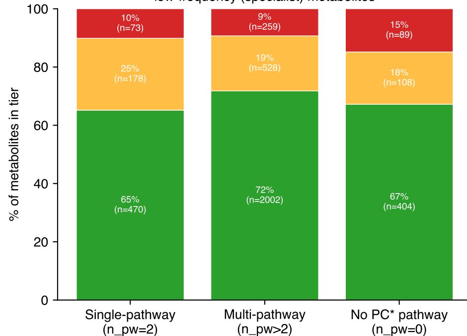
B. Coverage gap concentrates in low-frequency (specialist) metabolites
