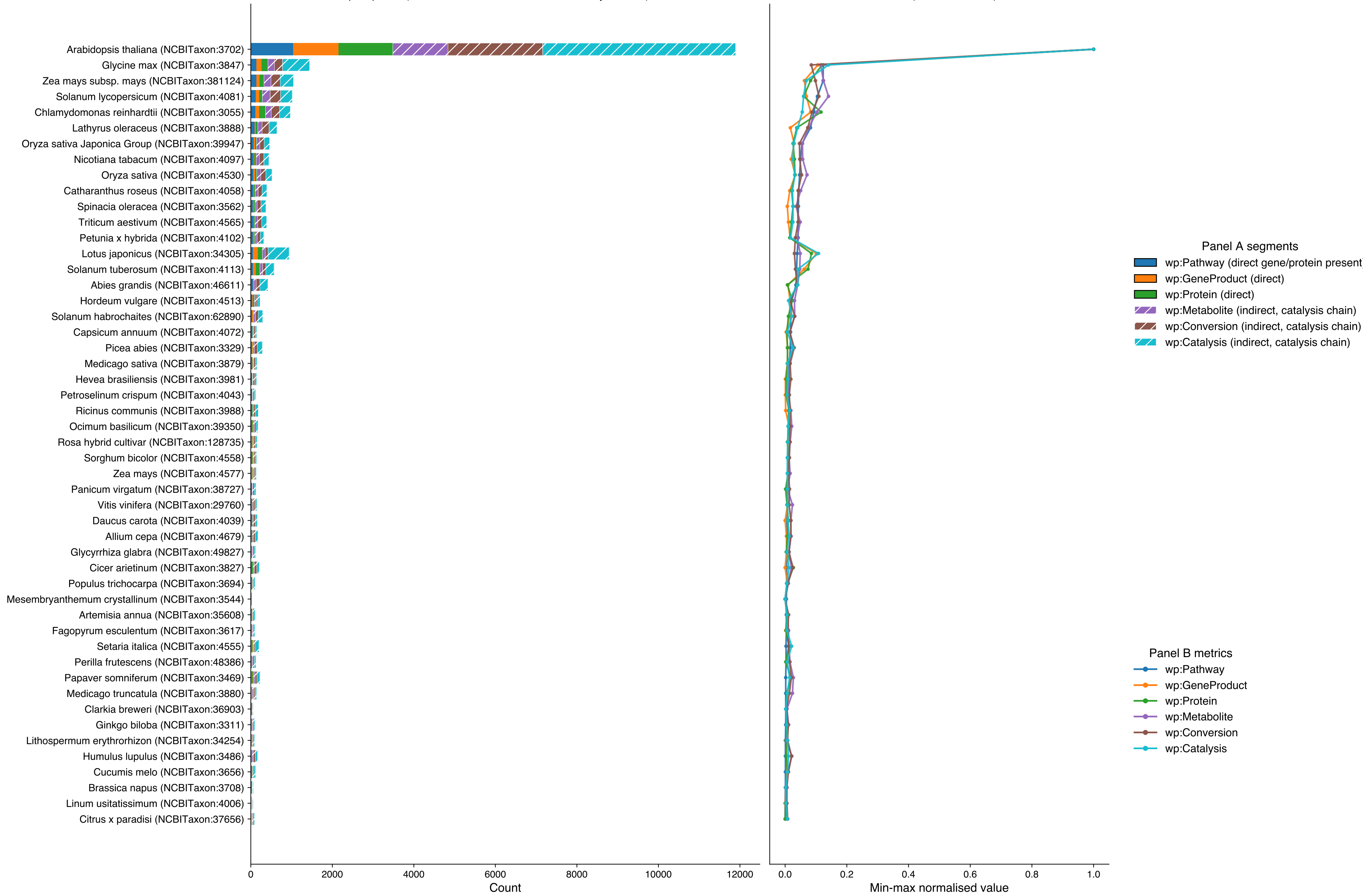
A -- Absolute counts per species (solid = direct, hatched = indirect via catalysis chain)
