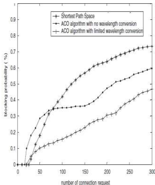
Fig. 5 ACO and shortest path
