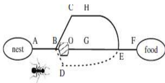
Fig. 2 The shortest path after initial searching time
