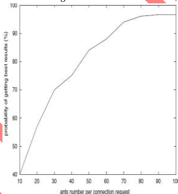
Fig. 6 Influence of different ant numbers to searching result
