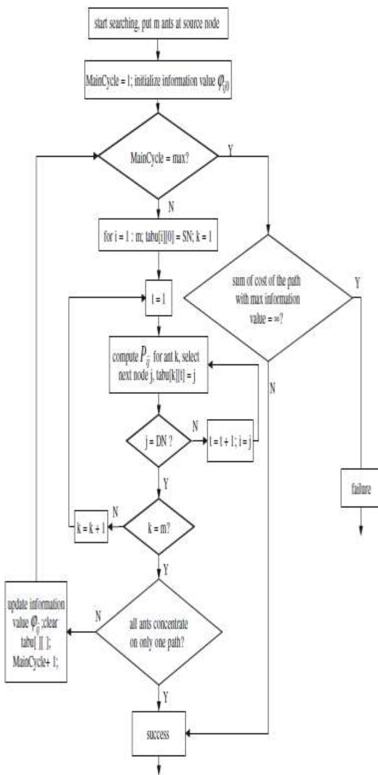
Fig. 3 ACO flowchart
