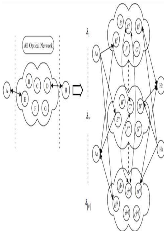
Fig. 1 Interconnected multilayer-graph model
