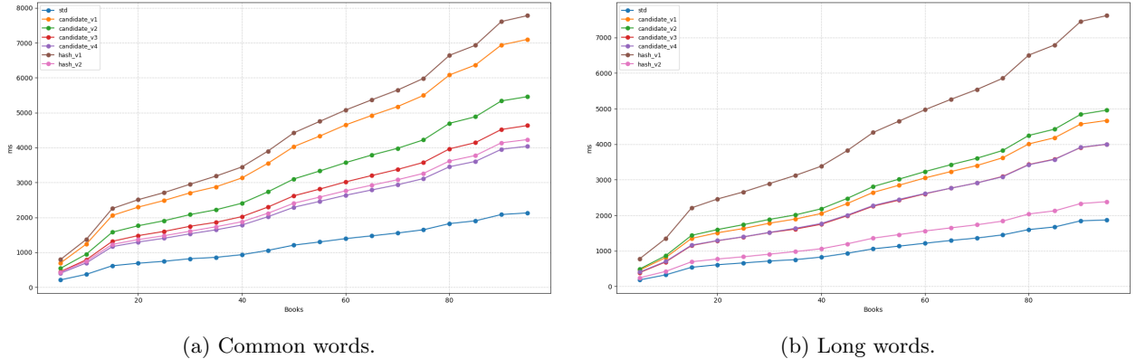
Figure 2: Runtime for sequential implementations for varying book counts (100 queries).
