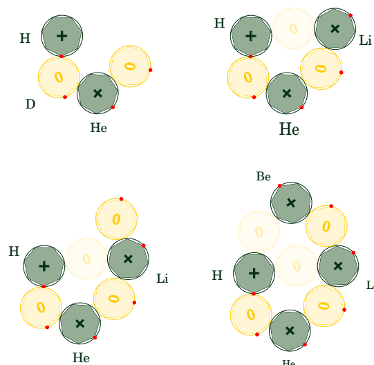
Figure 19: Step-by-step construction of atomic nuclei. The proton in green is linked with a neutron in yellow. The association is made by a shift of 2\pi/7 (traceable via the red dots), creating a spiral. To prevent the spiral from bursting due to electrical repulsion, it is necessary to shift the placement of a proton (light yellow) to link two non-consecutive protons. The first neutronic link is between the lithium proton and the hydrogen proton, the second between beryllium and hydrogen.
