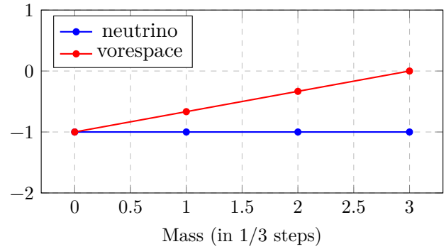
Neutrino-vospace charge competition
