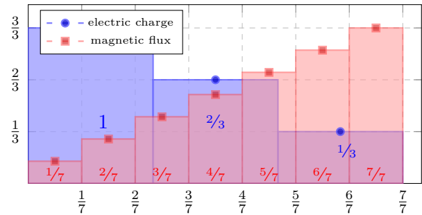
Vospace: electric charge vs magnetic flux
