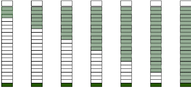
Figure 13: Mass distribution in a vorespaces. The vorespaces can be seen, according to the mass, as composed of 3 parts: 1 of 20 states corresponding to the equilibrium state (first white box), followed by 21 boxes representing each gravity-charge pair and finally the blocking state, in dark green. Fractality requires that the distribution be made in 7 jumps, therefore by a jump of 3 double pairs (in light green)
