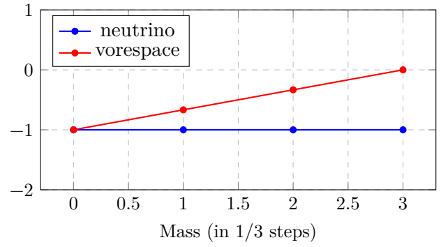
Neutrino-vospace charge competition
