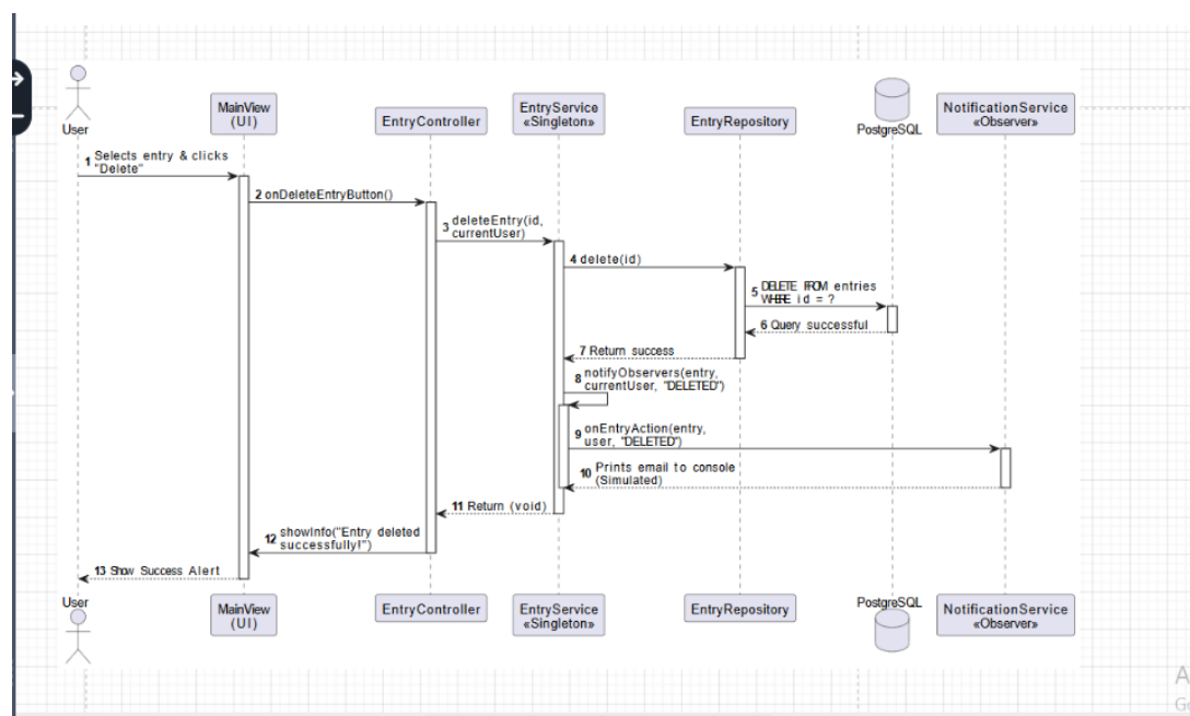
Figure 5: Sequence Diagram - Command Execution and Notification
