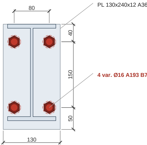
VISTA DE FRENTE ESC 1:5 c_plate + c_ishape + c_nut_front + c_leader
