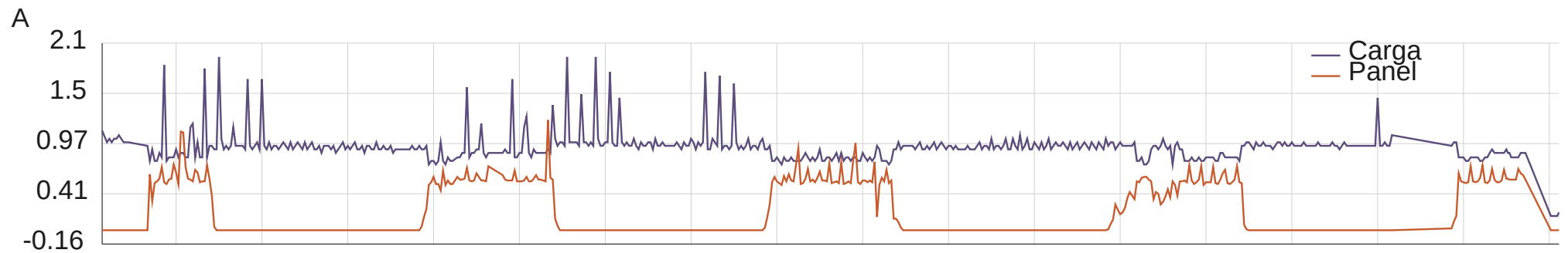
XTRA2210 - corrientes
