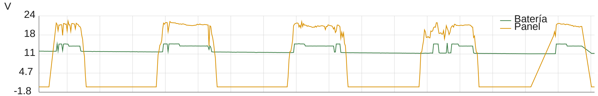
XTRA2210 - tensiones
