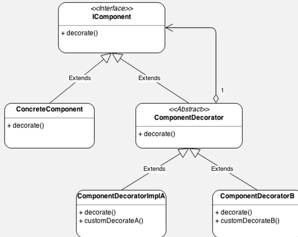
Decorator pattarn – Class diagram
