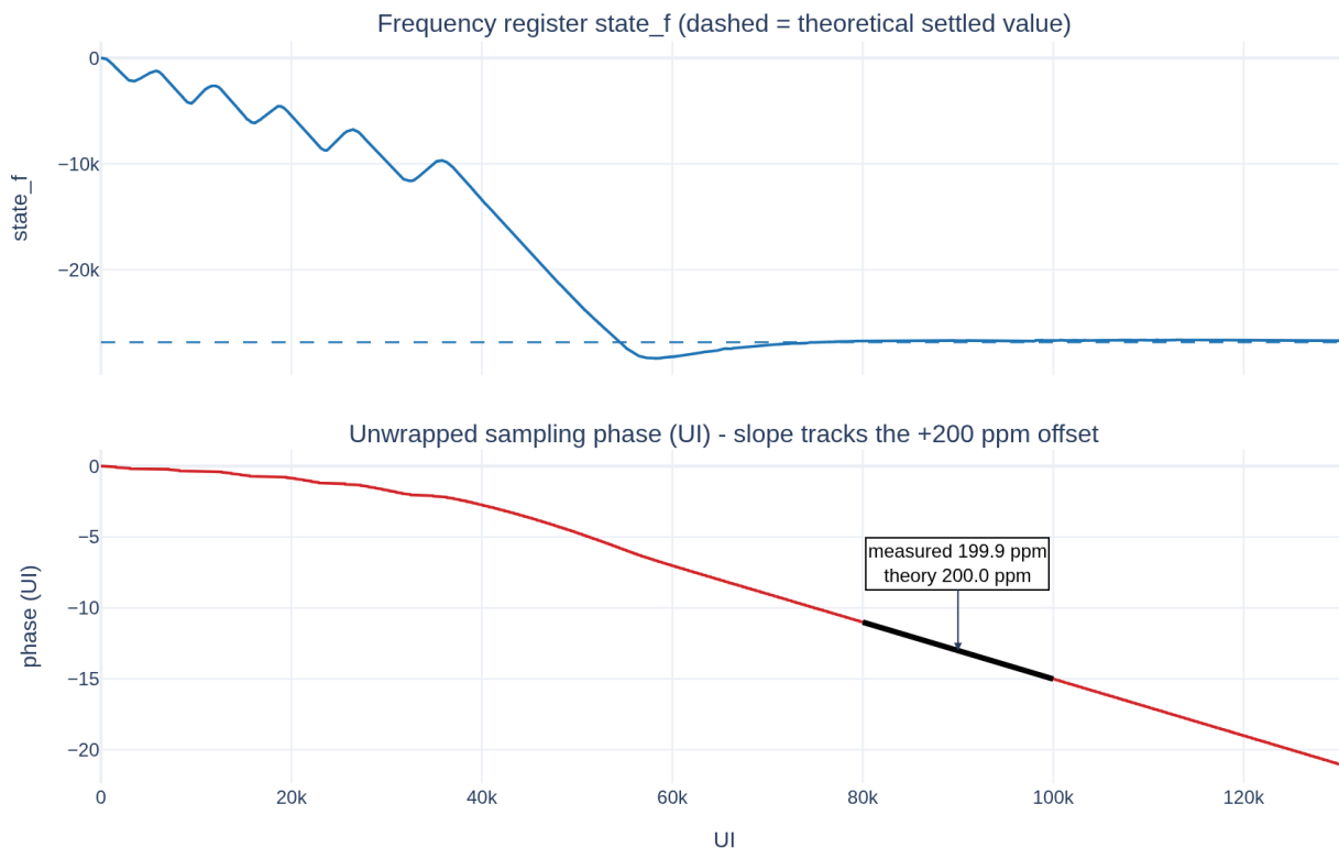
Figure 5-1: Closed-loop acquisition of a +200 ppm frequency offset at the default loop gains. Top: the frequency register \text{state\_f} slews from 0 and settles onto the theoretical value (dashed) after ~56k UI.
