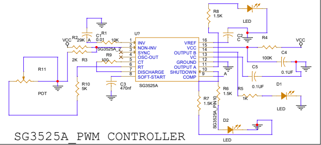
SG3525A_PWM_CONTROLLER
