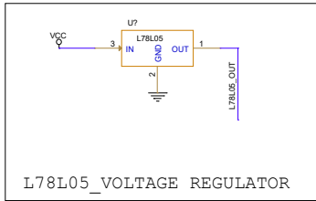
L78L05_VOLTAGE REGULATOR
