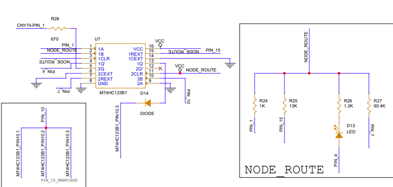
DUAL RETRIGGERABLE MONOSTABLE MULTIVIBRATOR-M74HC123B1
