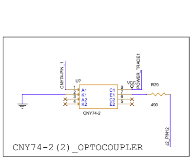
CNY74-2 (2)_OPTOCOUPLER
