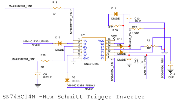
SN74HC14N -Hex Schmitt Trigger Inverter
