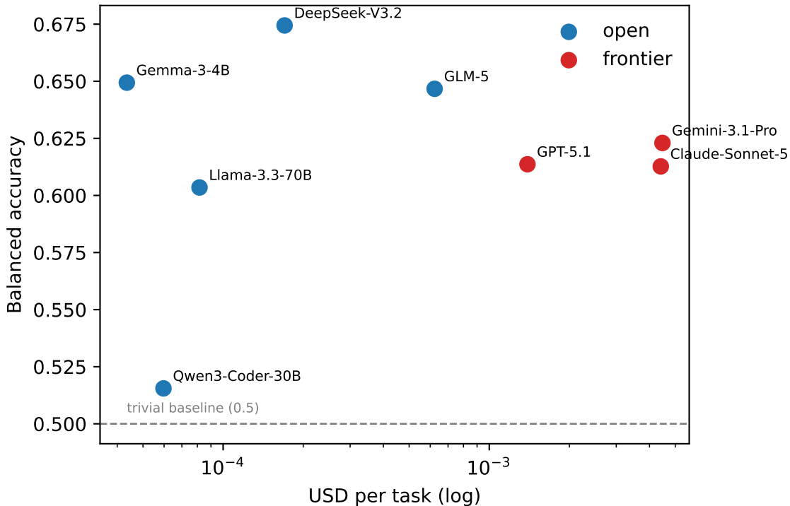
Detection quality vs USD per task (log)
