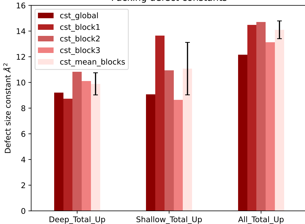
Packing defect constants
