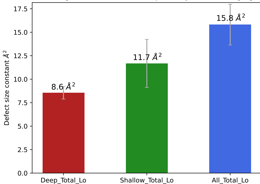
Packing defect constants computed by block averaging
