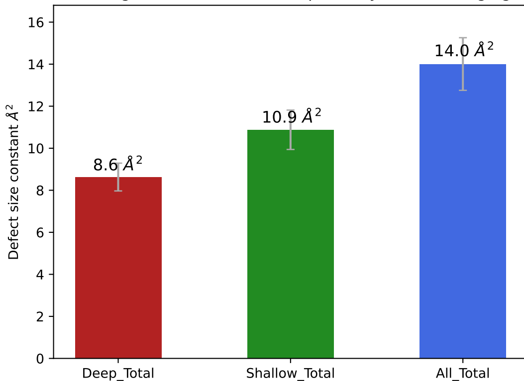
Packing defect constants computed by block averaging
