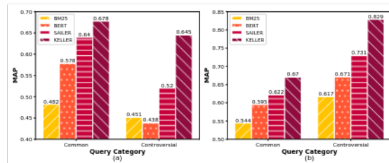
Figure 3: Evaluation on different query types. We evaluate four models on (a) LeCaRD and (b) LeCaRDv2.
