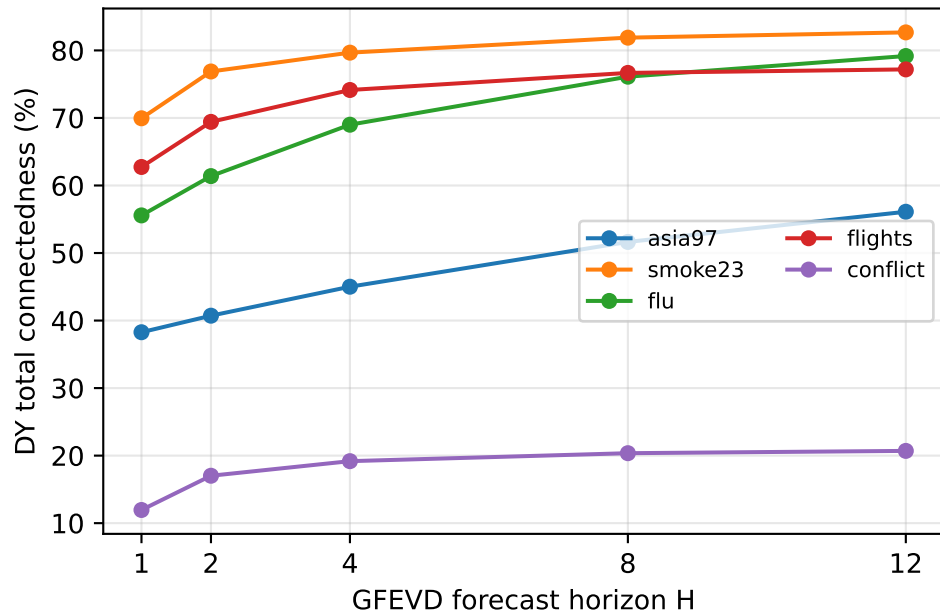
(a) DY total connectedness vs horizon
