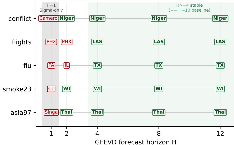
(b) Net-transmitter identity vs horizon (green = matches published H=10 transmitter)
